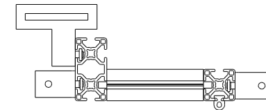
VIEW D-D
