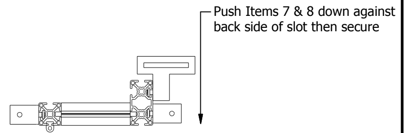
VIEW C-C
